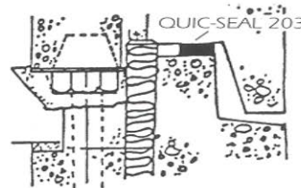
Detail: Precast Parapet Fixing
