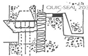
Detail: Precast Parapet Fixing
