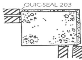
Plan: Brick To Column Detail
